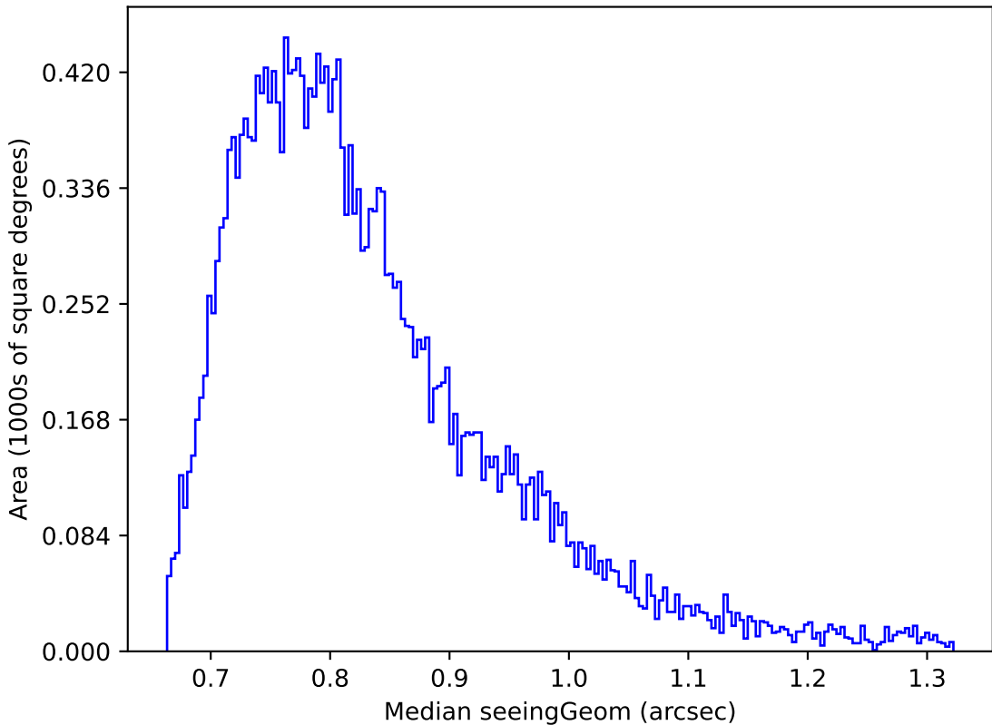
ddf_loaded_fl15_v3.4_10yrs Yr 1 i band: Median seeingGeom
