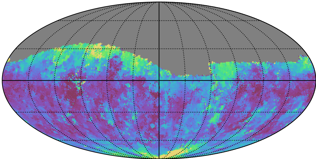
ddf_loaded_fl15_v3.4_10yrs Yr 1 g band: Median seeingGeom
