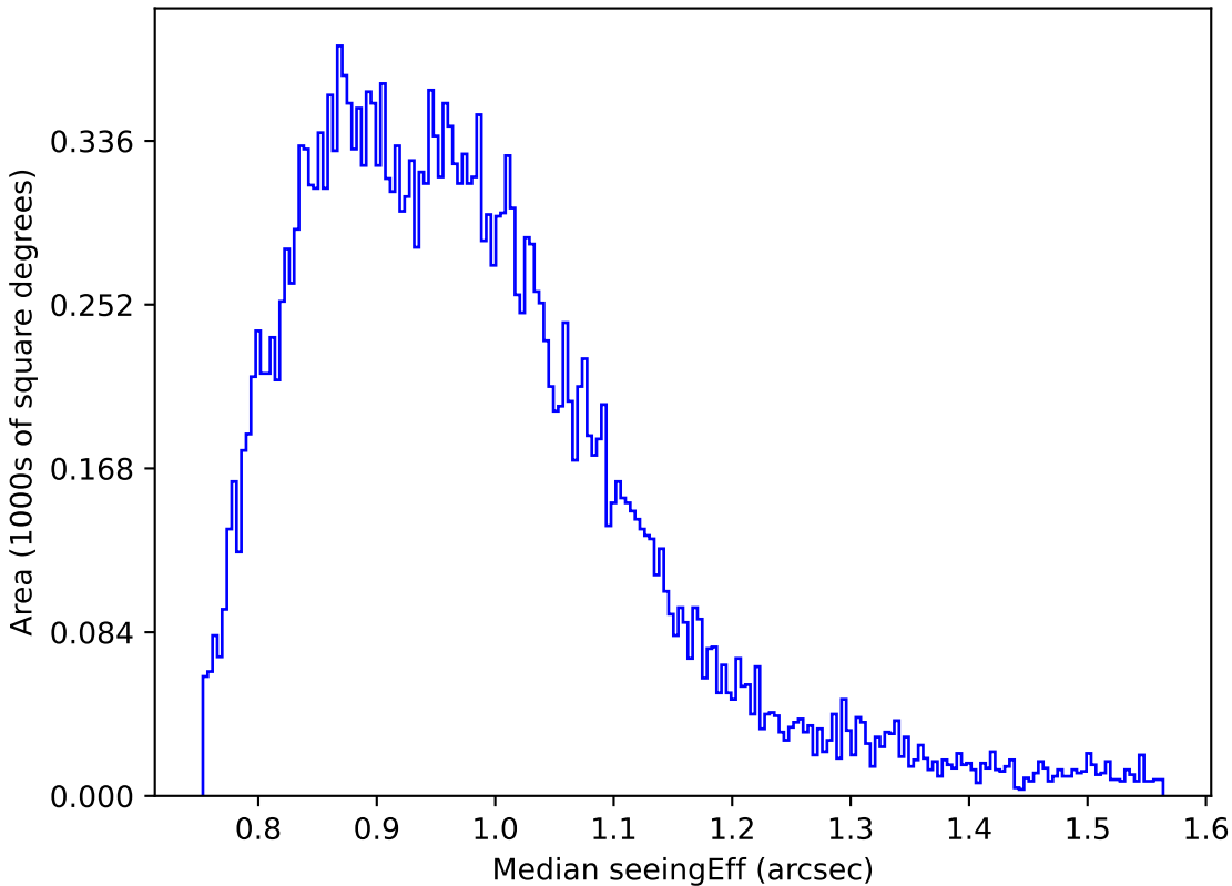
ddf_loaded_fl15_v3.4_10yrs Yr 1 z band: Median seeingEff
