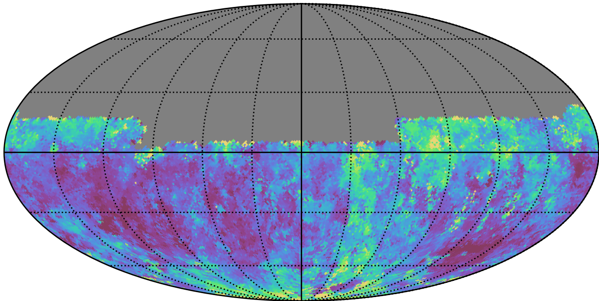
ddf_loaded_fl15_v3.4_10yrs Yr 1 y band: Median seeingEff
