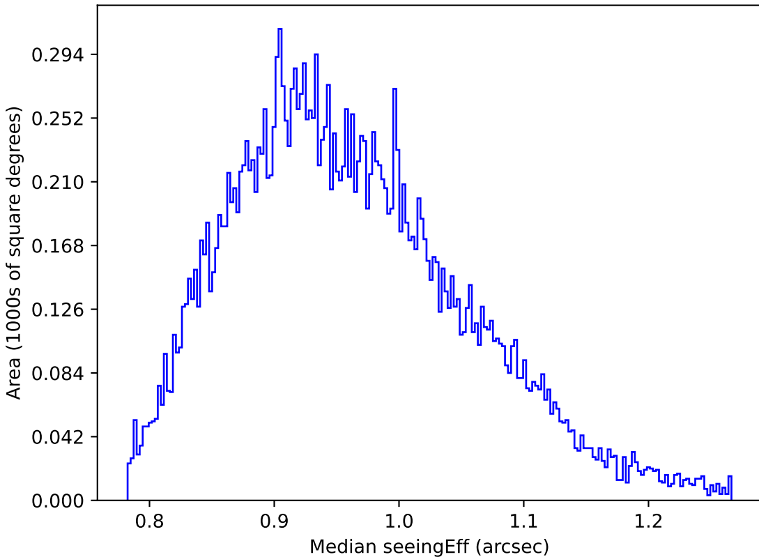
ddf_loaded_fl15_v3.4_10yrs Yr 1 y band: Median seeingEff
