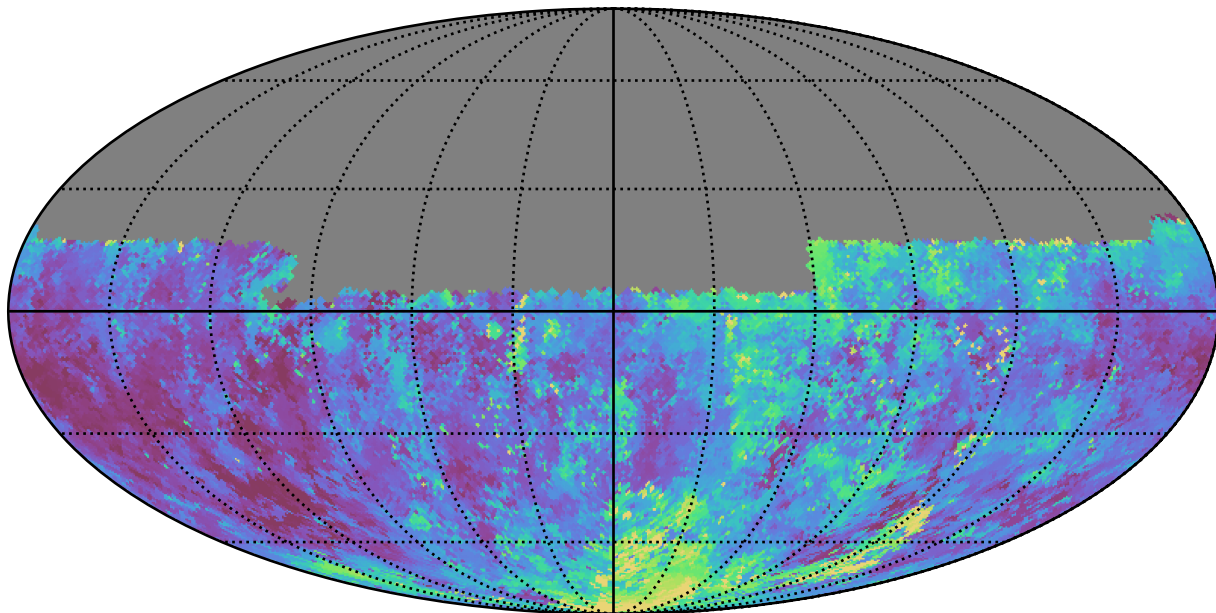
ddf_loaded_fl15_v3.4_10yrs Yr 1 u band: Median seeingEff
