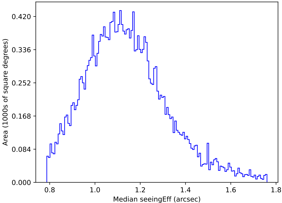
ddf_loaded_fl15_v3.4_10yrs Yr 1 u band: Median seeingEff
