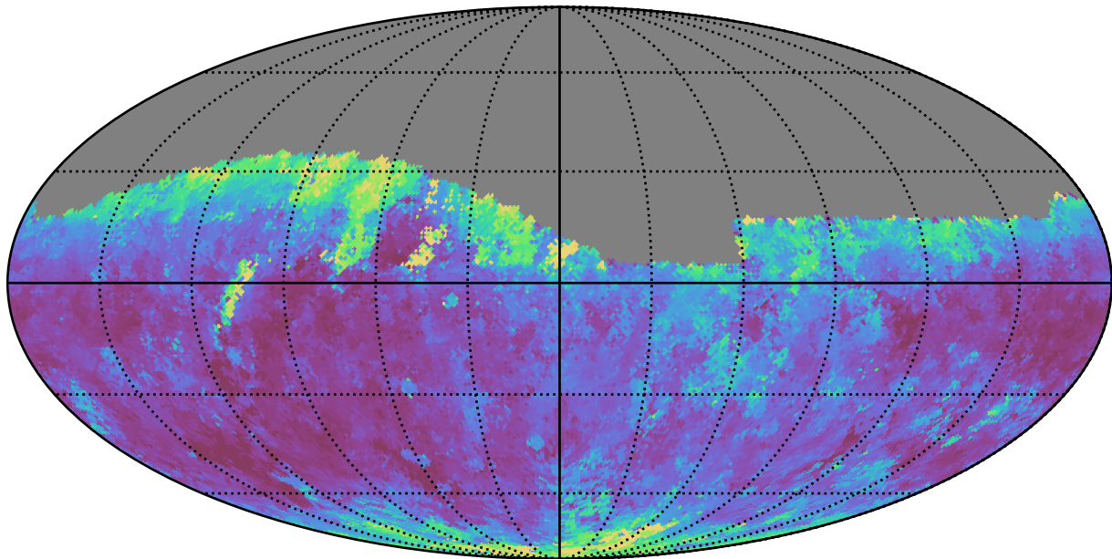
ddf_loaded_fl15_v3.4_10yrs Yr 1 r band: Median seeingEff
