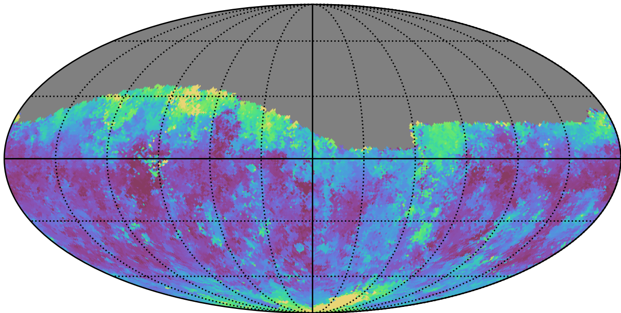
ddf_loaded_fl15_v3.4_10yrs Yr 1 g band: Median seeingEff
