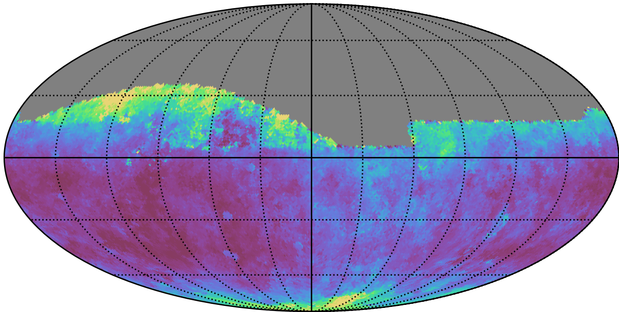
ddf_loaded_fl15_v3.4_10yrs Yr 1 all bands: Median seeingEff
