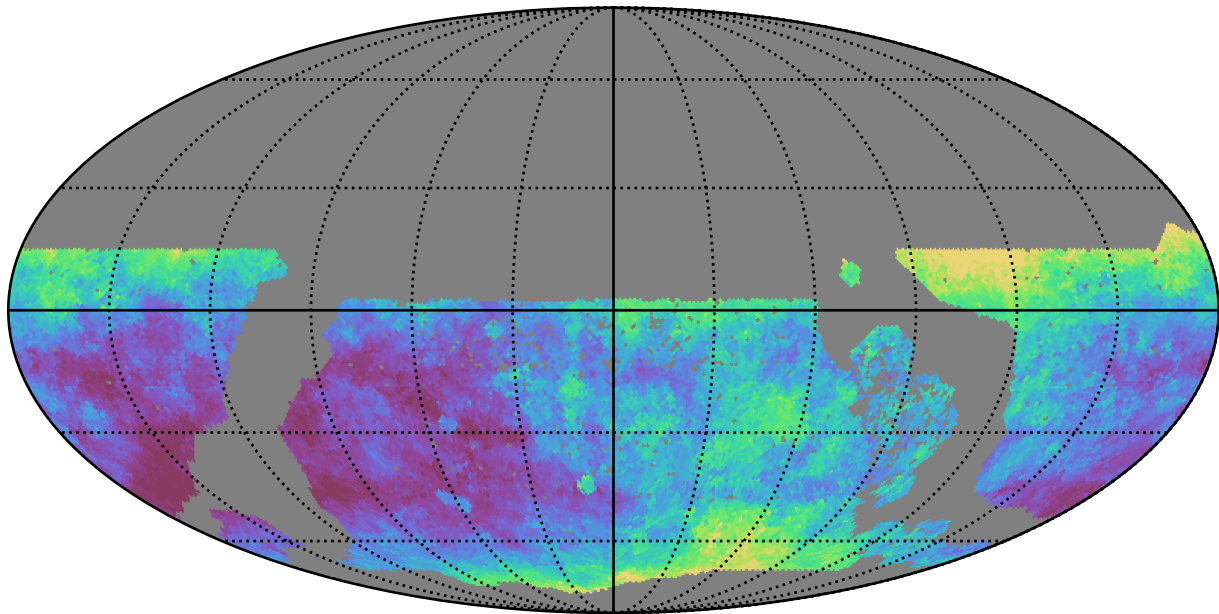
ddf_loaded_fl15_v3.4_10yrs WFD z band: Median seeingEff
