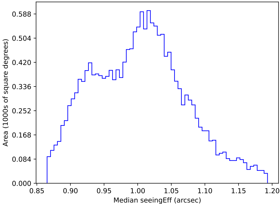
ddf_loaded_fl15_v3.4_10yrs WFD z band: Median seeingEff
