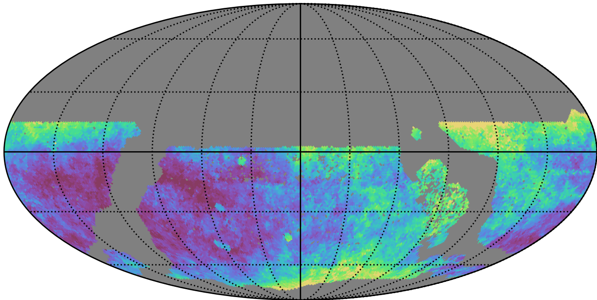
ddf_loaded_fl15_v3.4_10yrs WFD y band: Median seeingEff
