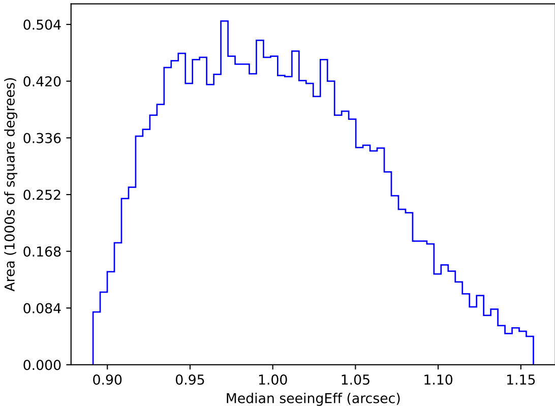
ddf_loaded_fl15_v3.4_10yrs WFD y band: Median seeingEff
