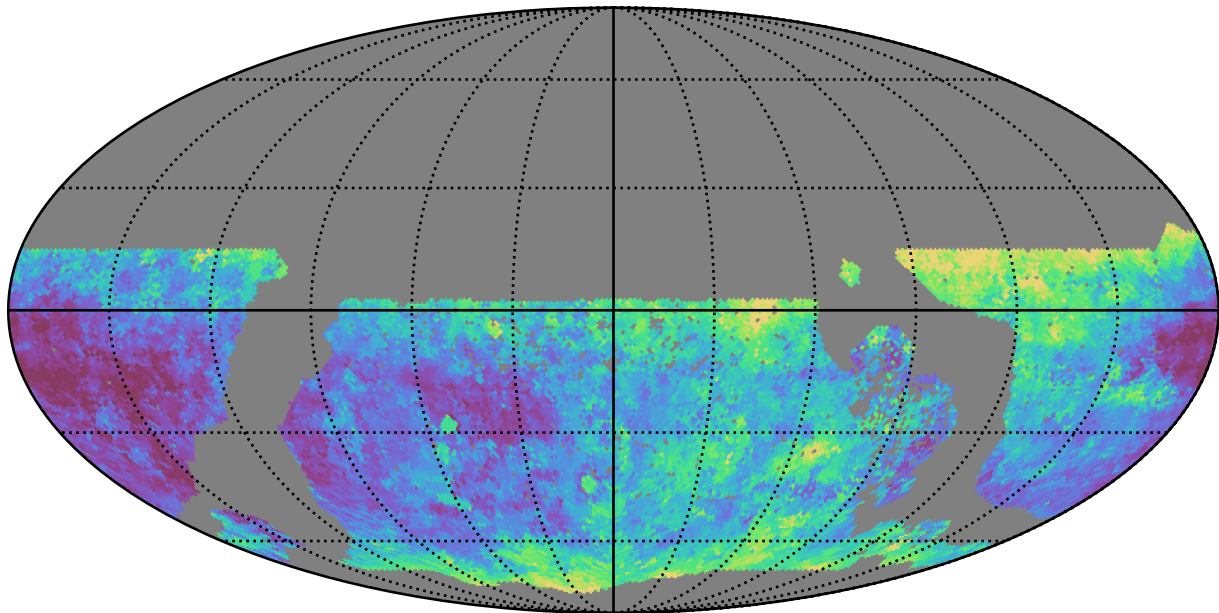
ddf_loaded_fl15_v3.4_10yrs WFD u band: Median seeingEff
