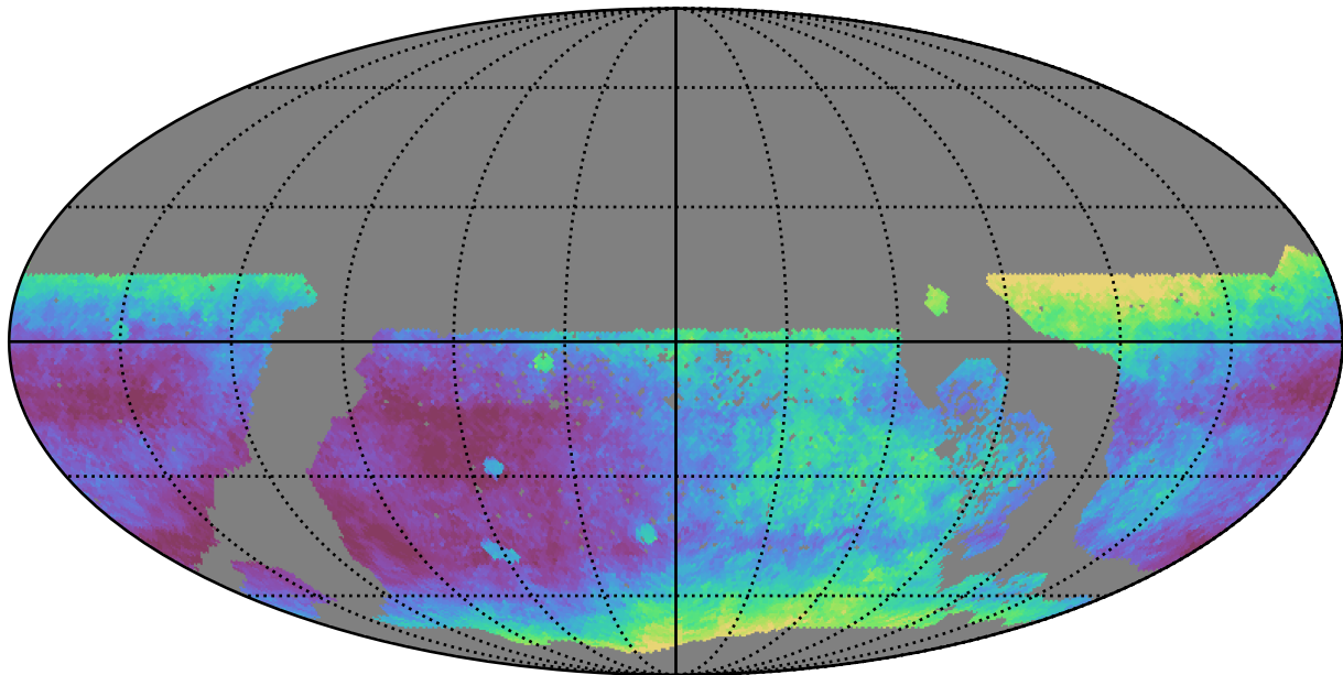
ddf_loaded_fl15_v3.4_10yrs WFD r band: Median seeingEff
