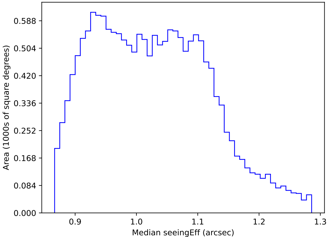
ddf_loaded_fl15_v3.4_10yrs WFD r band: Median seeingEff
