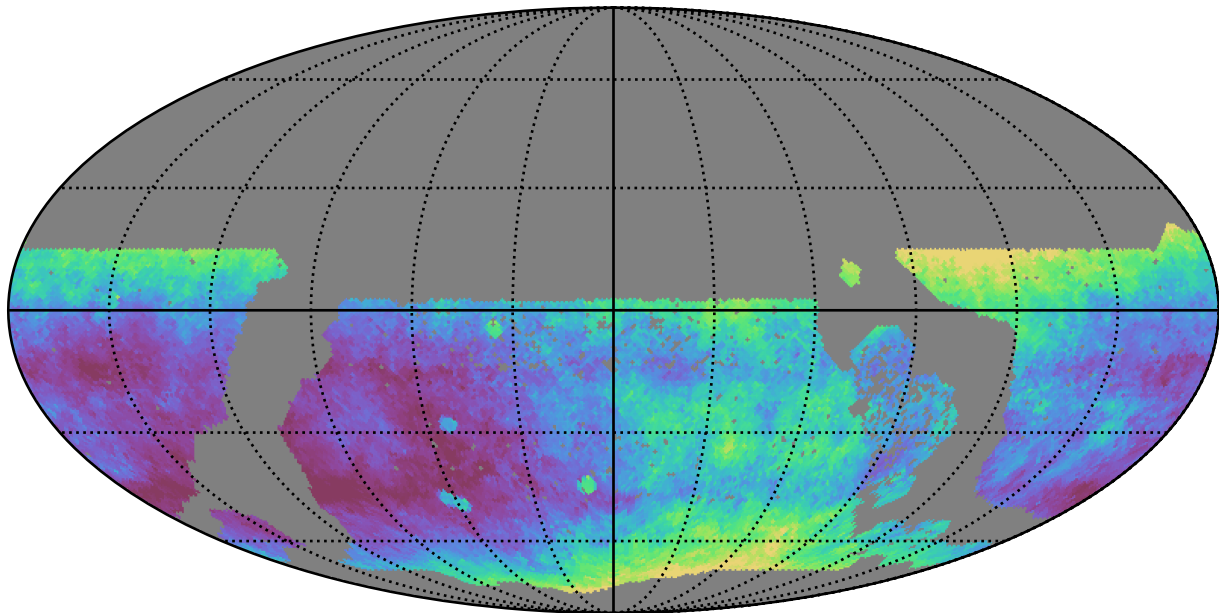
ddf_loaded_fl15_v3.4_10yrs WFD i band: Median seeingEff
