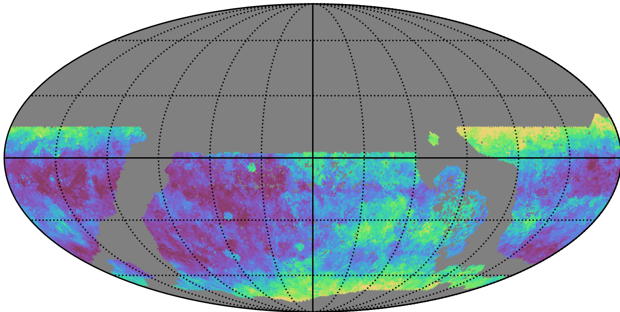
ddf_loaded_fl15_v3.4_10yrs WFD g band: Median seeingEff
