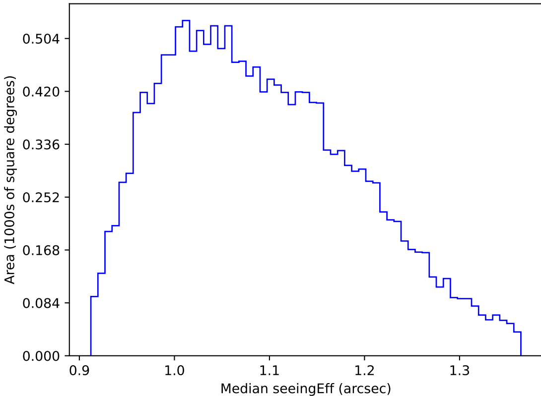
ddf_loaded_fl15_v3.4_10yrs WFD g band: Median seeingEff
