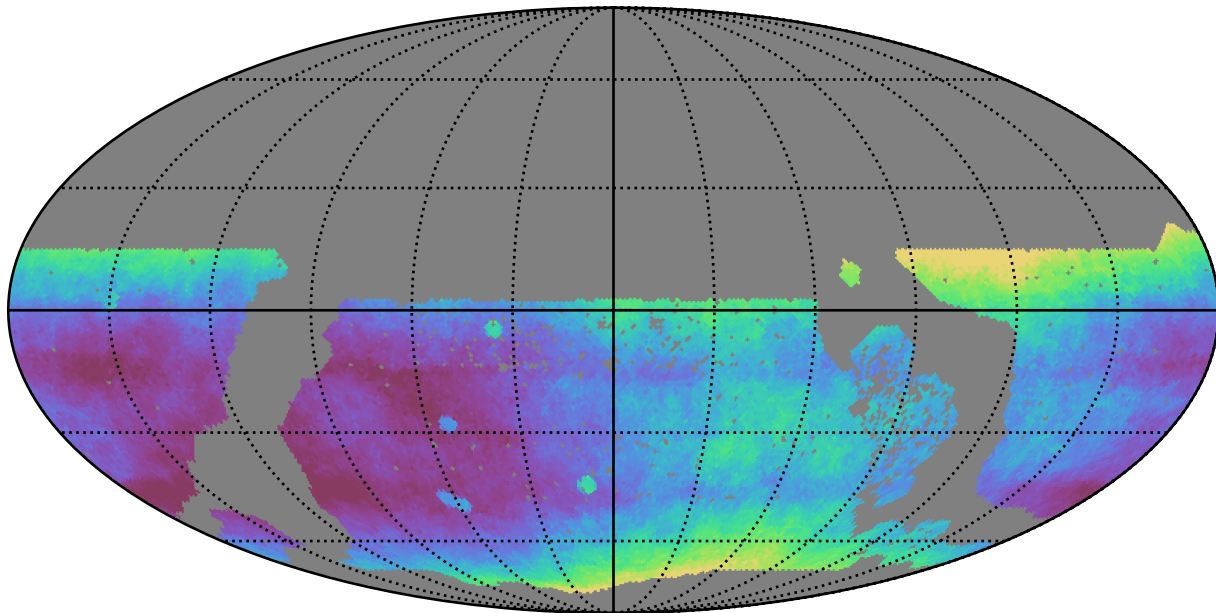
ddf_loaded_fl15_v3.4_10yrs WFD all bands: Median seeingEff
