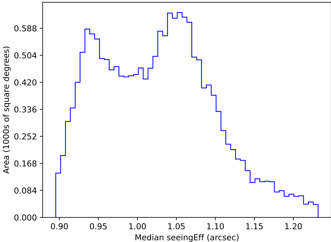
ddf_loaded_fl15_v3.4_10yrs WFD all bands: Median seeingEff
