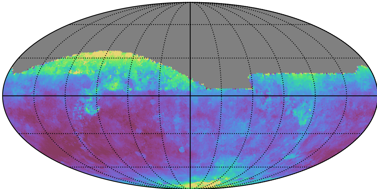
ddf_loaded_fl15_v3.4_10yrs All sky z band: Median seeingEff
