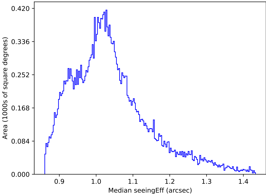
ddf_loaded_fl15_v3.4_10yrs All sky z band: Median seeingEff
