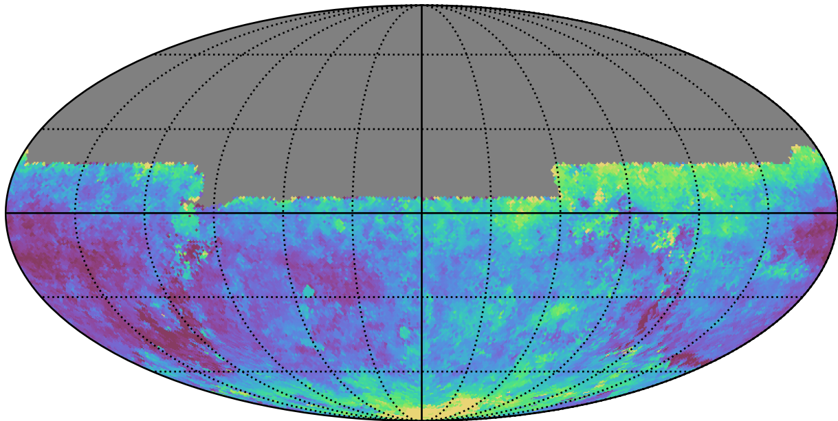
ddf_loaded_fl15_v3.4_10yrs All sky u band: Median seeingEff
