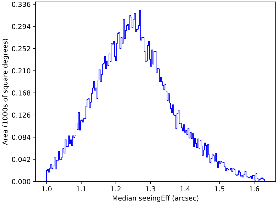
ddf_loaded_fl15_v3.4_10yrs All sky u band: Median seeingEff
