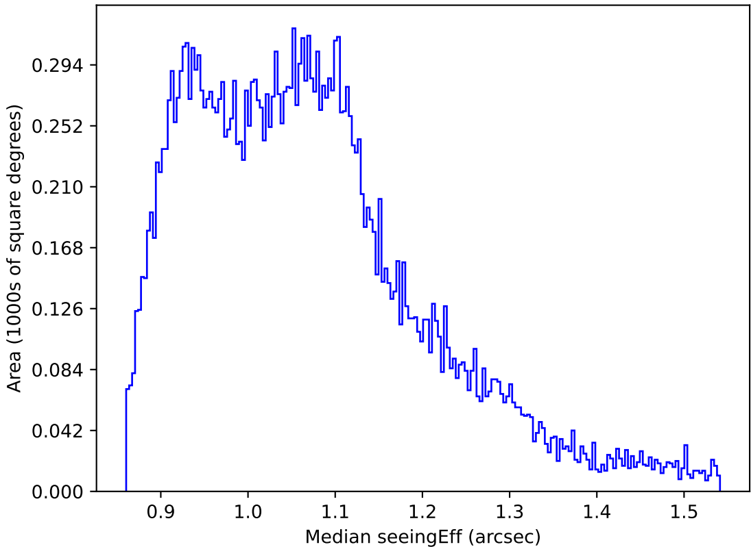
ddf_loaded_fl15_v3.4_10yrs All sky r band: Median seeingEff
