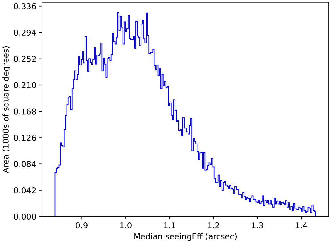
ddf_loaded_fl15_v3.4_10yrs All sky i band: Median seeingEff
