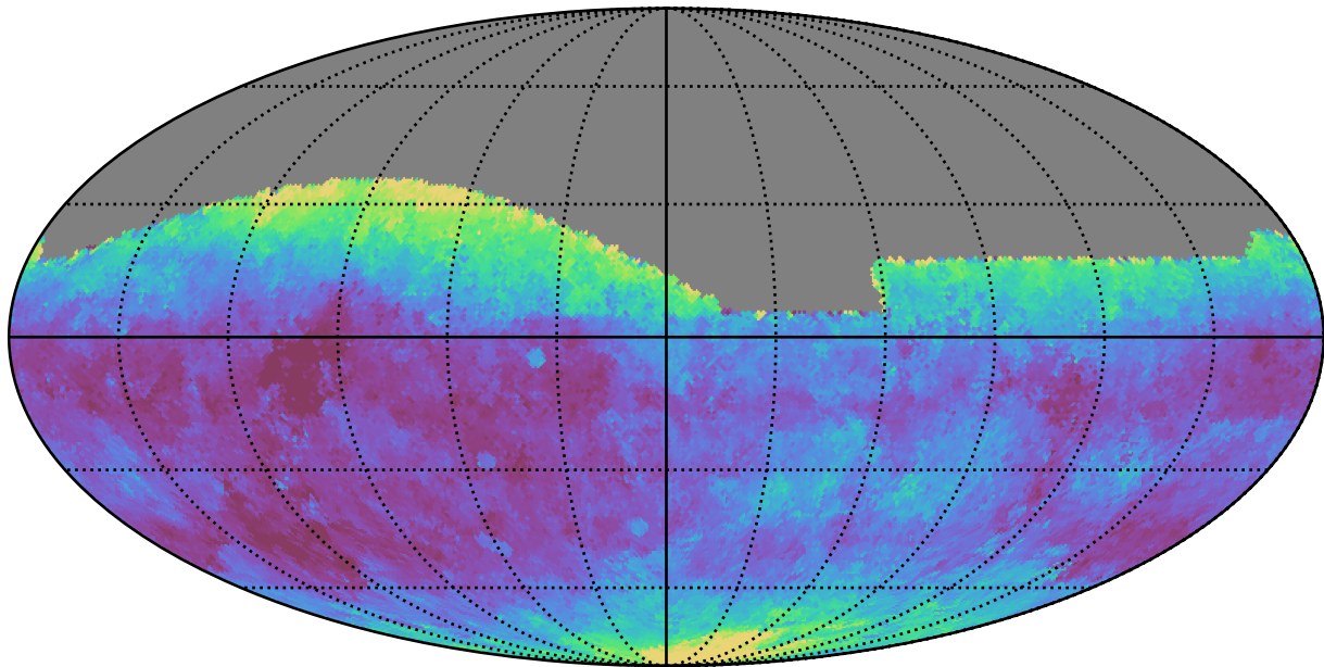
ddf_loaded_fl15_v3.4_10yrs All sky g band: Median seeingEff
