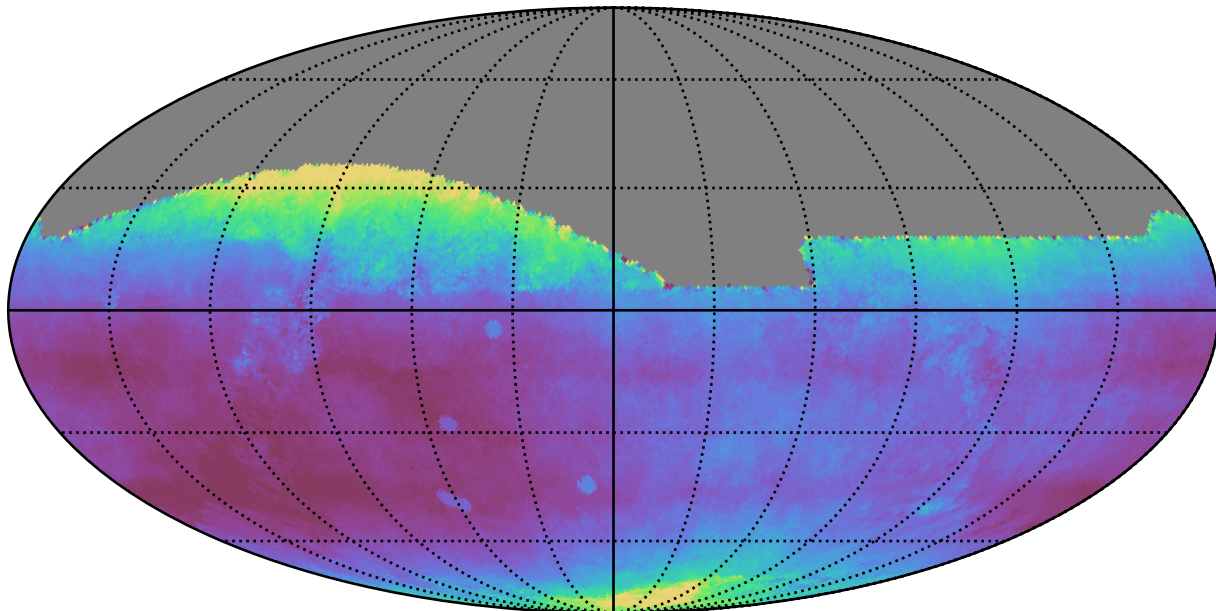
ddf_loaded_fl15_v3.4_10yrs All sky all bands: Median seeingEff
