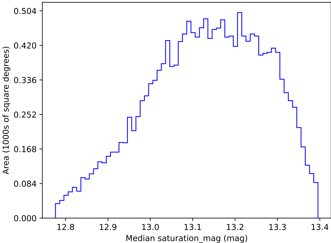
ddf_loaded_fl15_v3.4_10yrs WFD y band: Median saturation_mag
