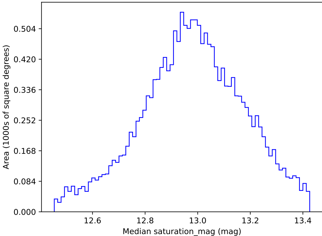
ddf_loaded_fl15_v3.4_10yrs WFD u band: Median saturation_mag
