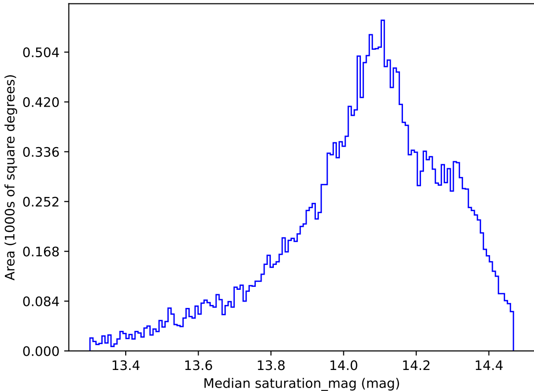
ddf_loaded_fl15_v3.4_10yrs All sky z band: Median saturation_mag
