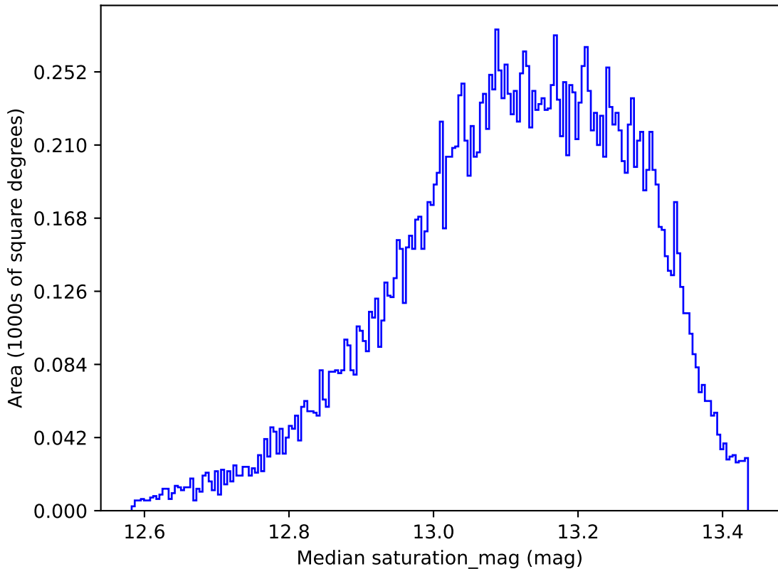
ddf_loaded_fl15_v3.4_10yrs All sky y band: Median saturation_mag
