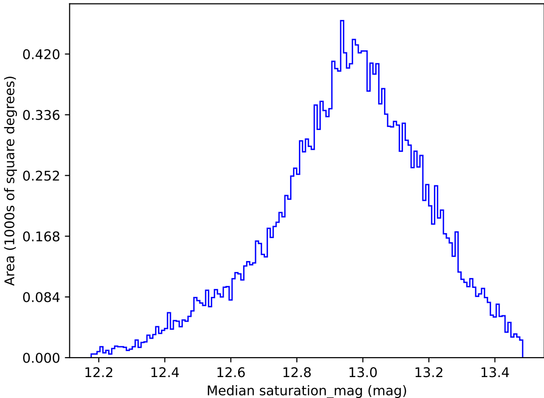
ddf_loaded_fl15_v3.4_10yrs All sky u band: Median saturation_mag
