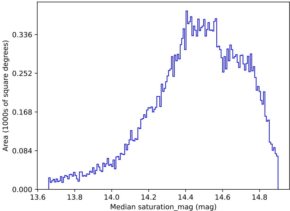
ddf_loaded_fl15_v3.4_10yrs All sky i band: Median saturation_mag
