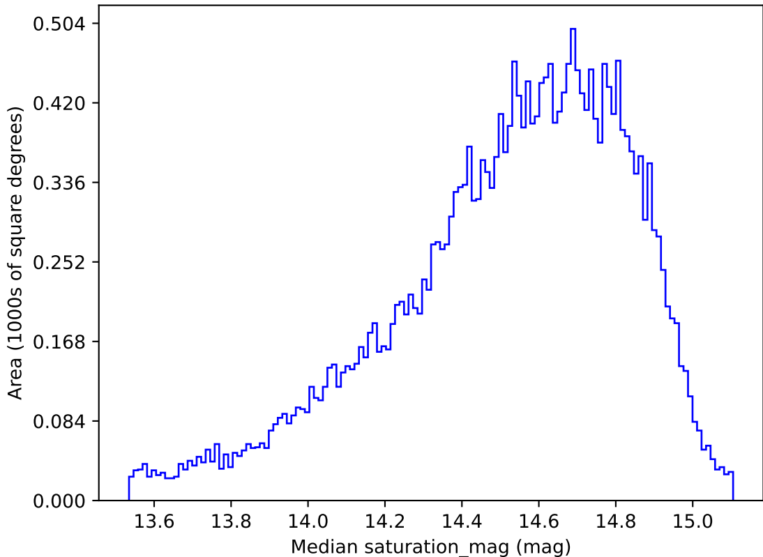
ddf_loaded_fl15_v3.4_10yrs All sky g band: Median saturation_mag
