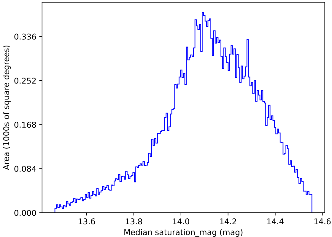
ddf_loaded_fl15_v3.4_10yrs All sky all bands: Median saturation_mag
