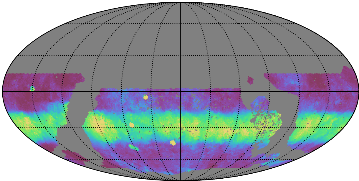
ddf_loaded_fl15_v3.4_10yrs WFD z band: Median normairmass
