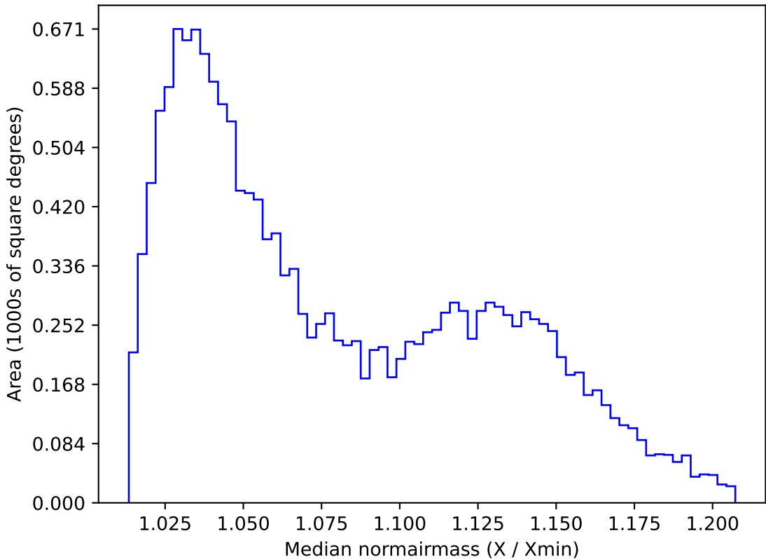
ddf_loaded_fl15_v3.4_10yrs WFD u band: Median normairmass
