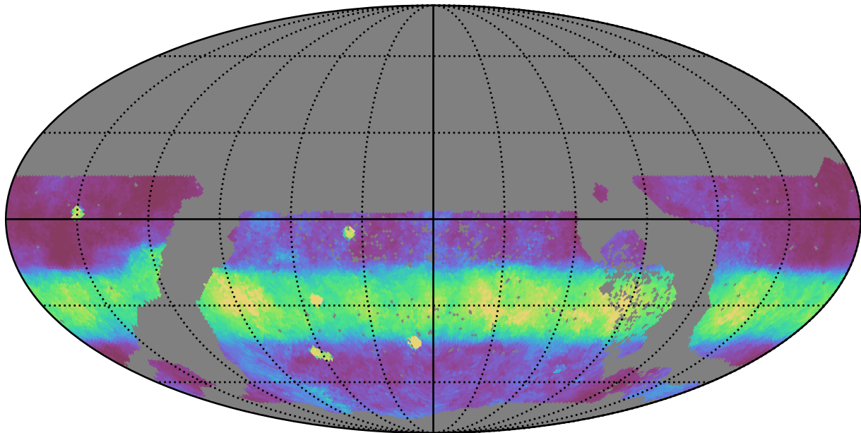
ddf_loaded_fl15_v3.4_10yrs WFD r band: Median normairmass
