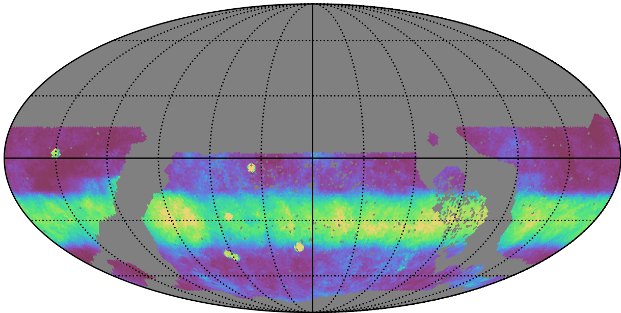
ddf_loaded_fl15_v3.4_10yrs WFD i band: Median normairmass
