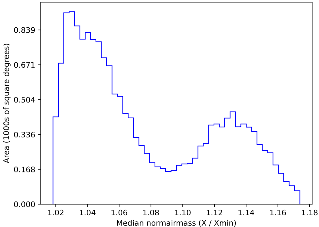
ddf_loaded_fl15_v3.4_10yrs WFD i band: Median normairmass
