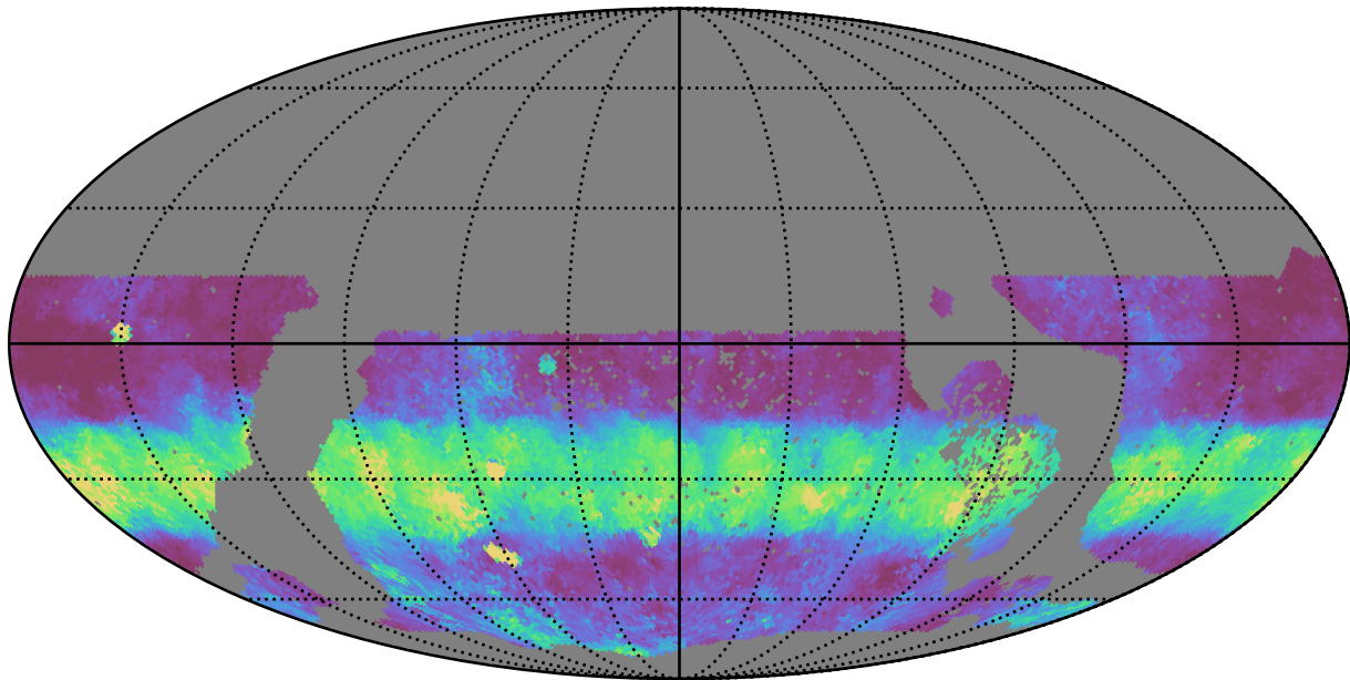
ddf_loaded_fl15_v3.4_10yrs WFD g band: Median normairmass
