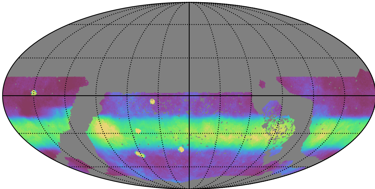
ddf_loaded_fl15_v3.4_10yrs WFD all bands: Median normairmass
