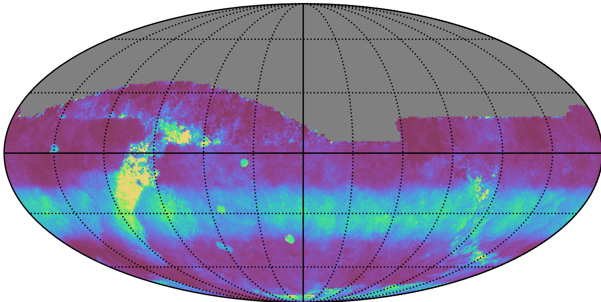
ddf_loaded_fl15_v3.4_10yrs All sky z band: Median normairmass
