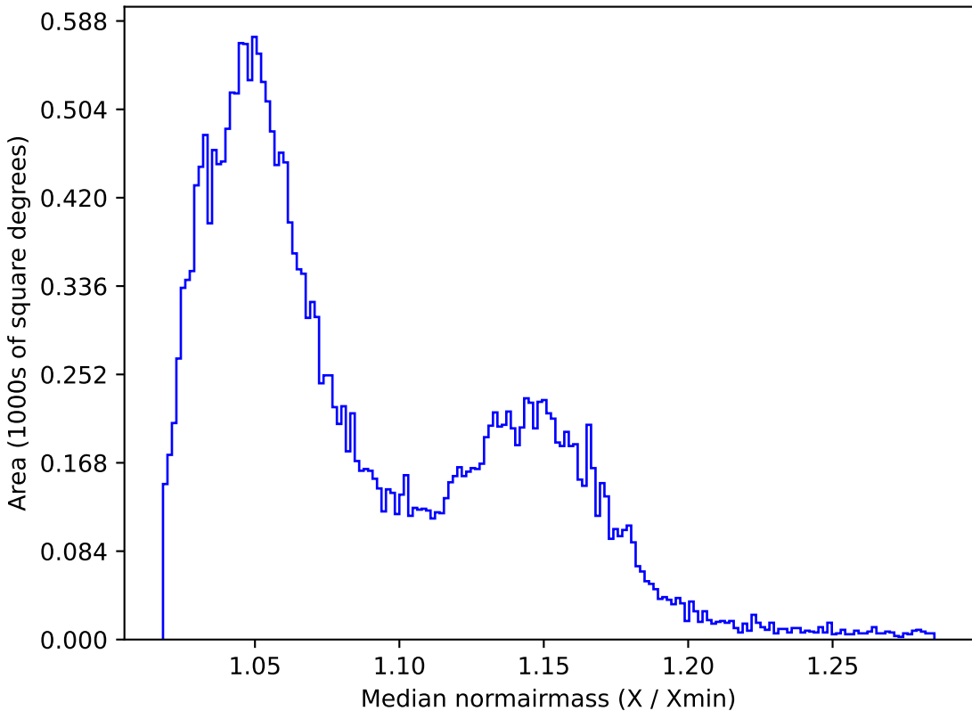
ddf_loaded_fl15_v3.4_10yrs All sky z band: Median normairmass
