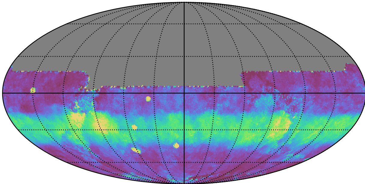
ddf_loaded_fl15_v3.4_10yrs All sky y band: Median normairmass
