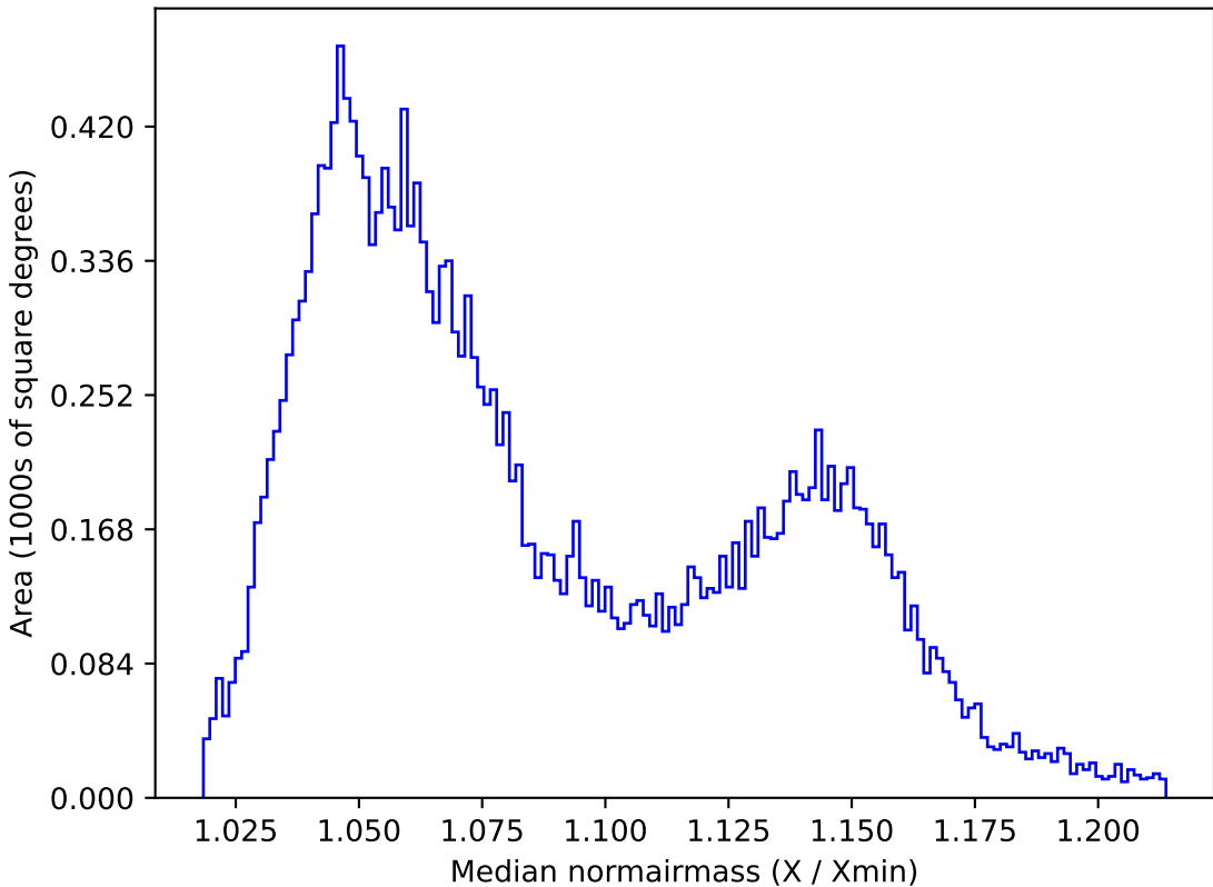
ddf_loaded_fl15_v3.4_10yrs All sky y band: Median normairmass
