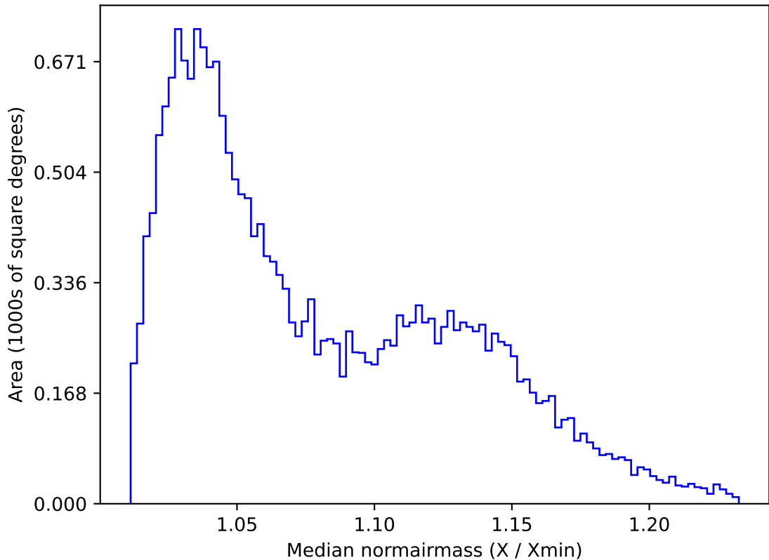
ddf_loaded_fl15_v3.4_10yrs All sky u band: Median normairmass
